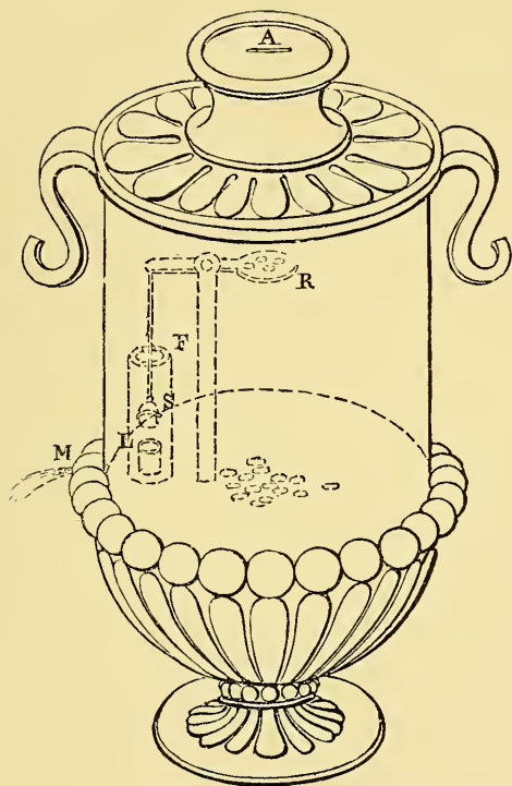
THE SLOT-MACHINE OF HERON
